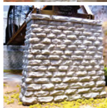
HO Single-Track Cut Stone Bridge Pier w/Rectangular Base Chooch. 214-8430 4-5/8 x 1 x 3-3/4" 11.7 x 2.5 x 9.5cm 214-8431 3-3/4 x 1 x 3-1/2" 9.5 x 2.5 x 8.9cm Reg. Price: $18.98 Sale: $16.98
